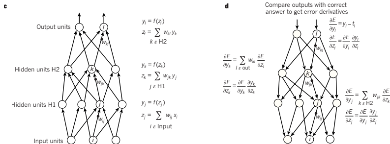
Fig. 9: To generally illustrate neural network training, consider a multilayer neural network with backpropagation [LeCun et al., 2015]. Training consists in iterating to minimize the loss.
