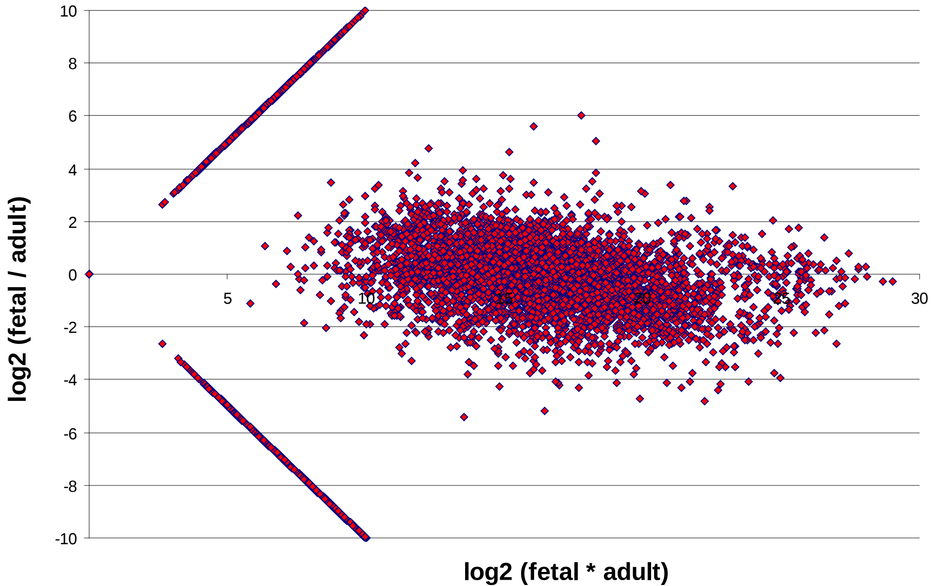
R-I plot for brain: fetal vs adult
